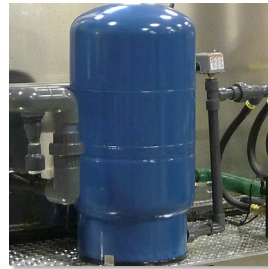
Pressure manifold set-up is standard on BIO-20R-0M11 and BIO-20R-1M11
